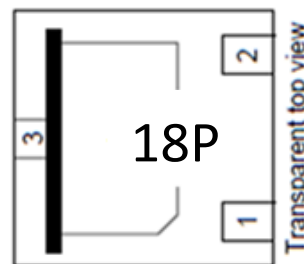
18P = Device Marking Code Bar denotes cathode
